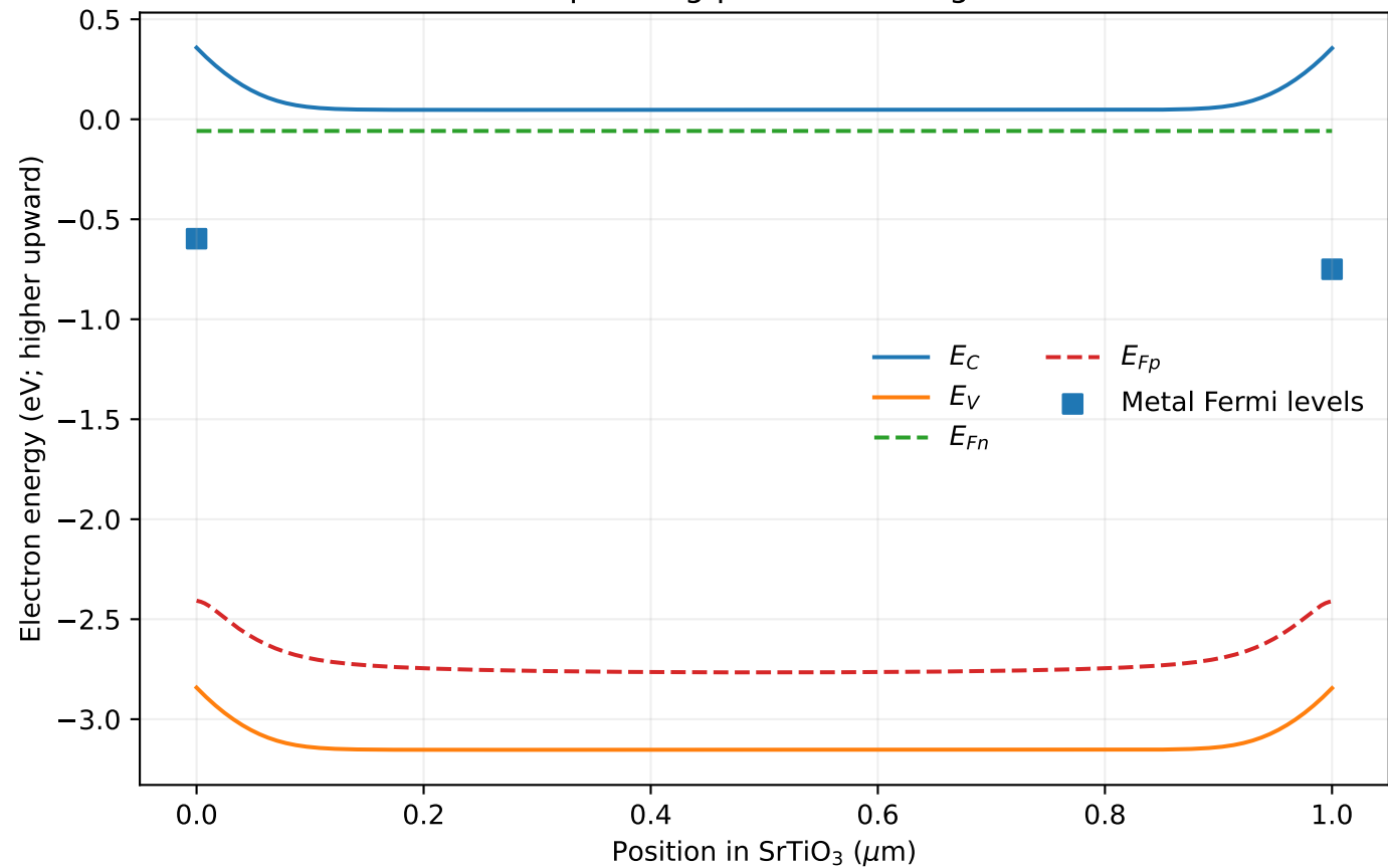
BB operating-point band diagram
