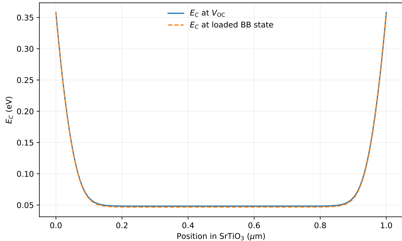
BB conduction-band profile: open circuit vs reverse-loaded state
