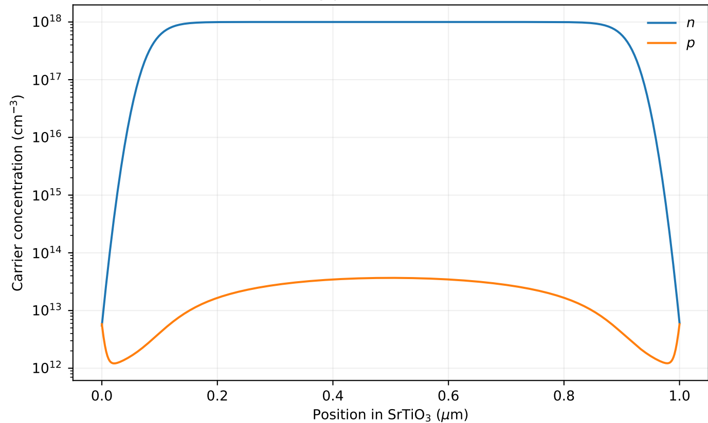
BB operating-point carrier concentrations
