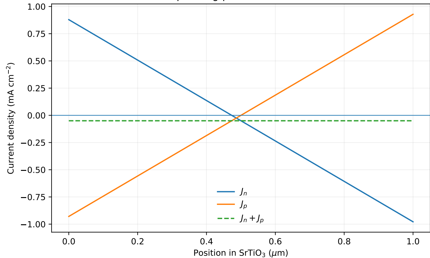
BB operating-point carrier currents
