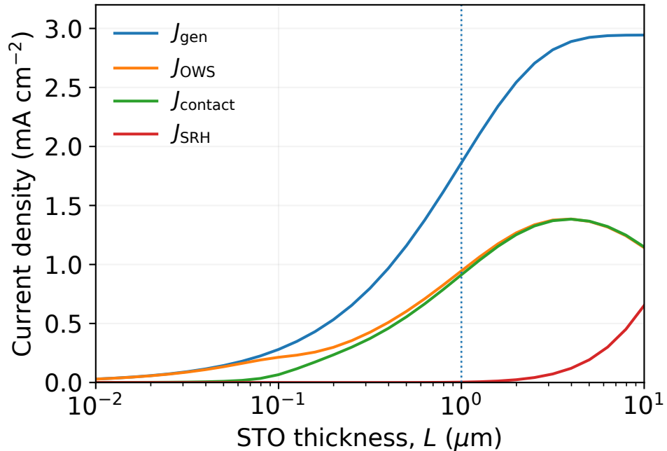
(a) Steady-state current balance
