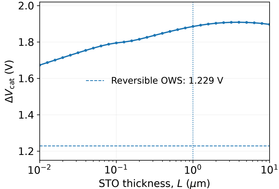
(b) Catalyst-potential separation
