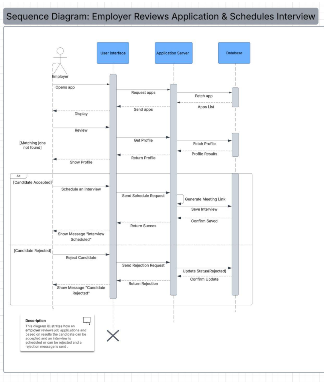
Figure 4: Sequence diagram (Employers)
