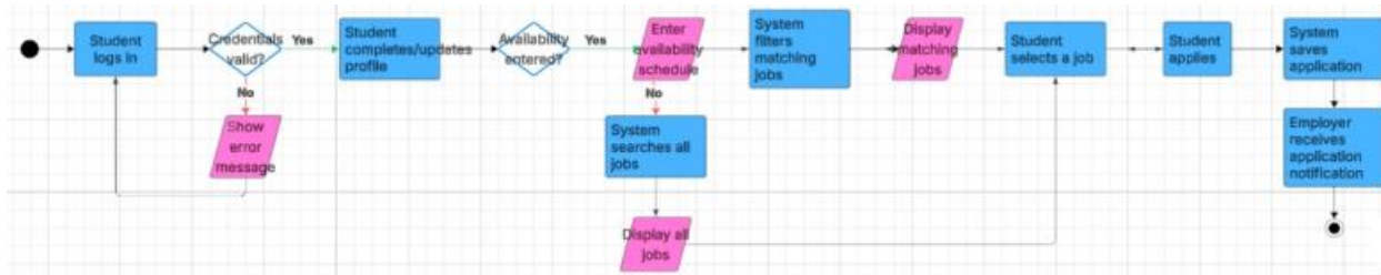
Figure 6: Activity diagram (Students)
