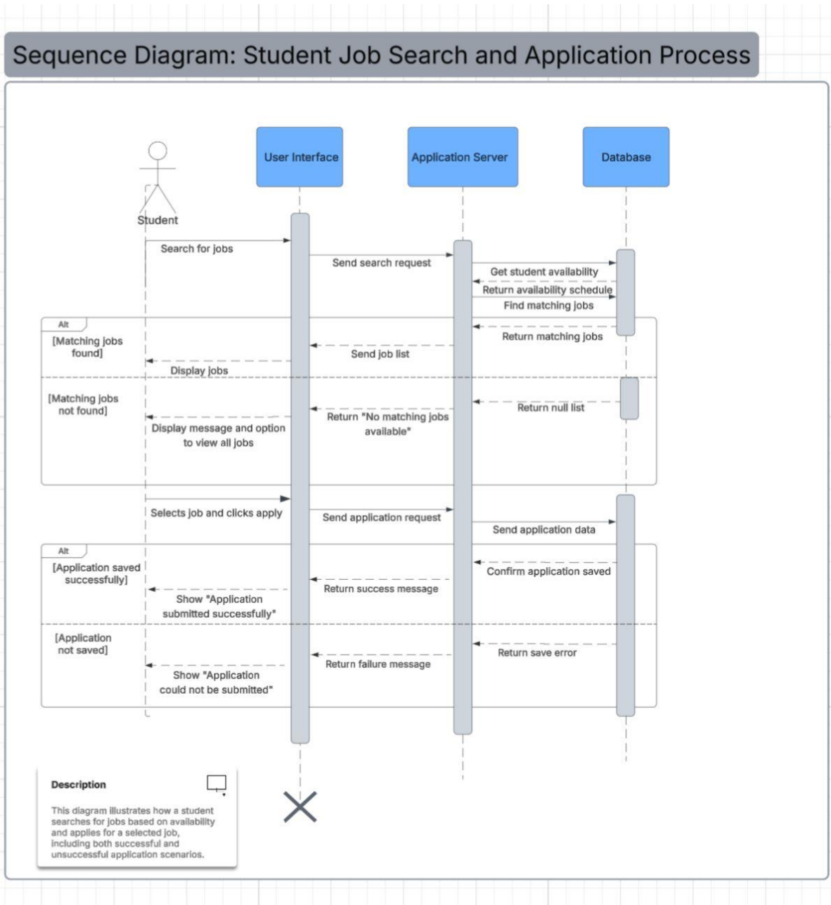
Figure 3: Sequence diagram (Students)
