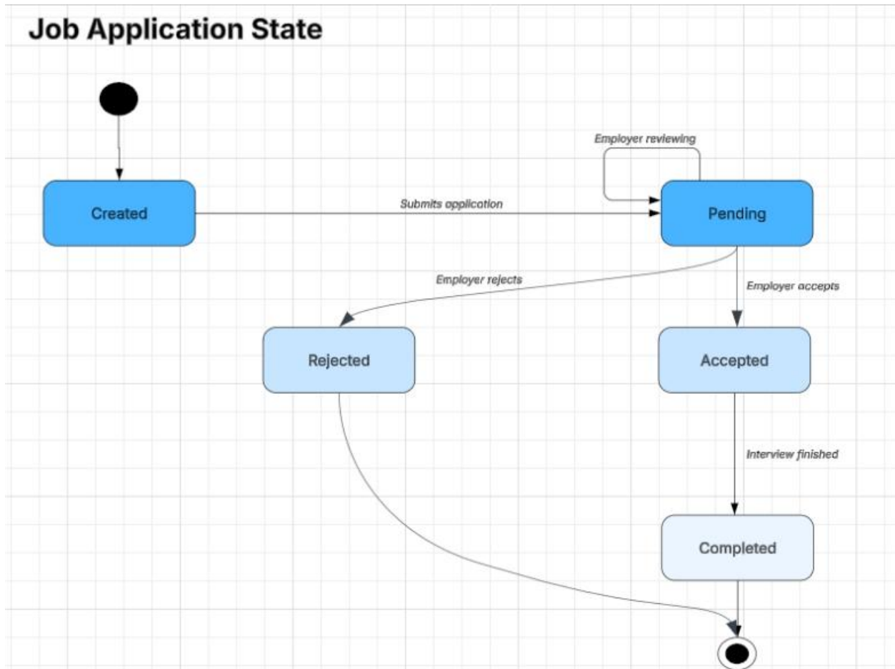
Figure 8: Job Application State Diagram
