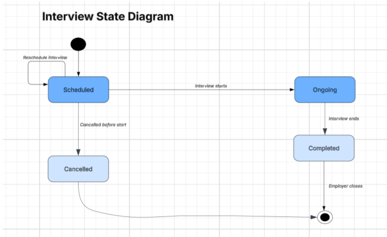
Figure 9: Interview State Diagram
