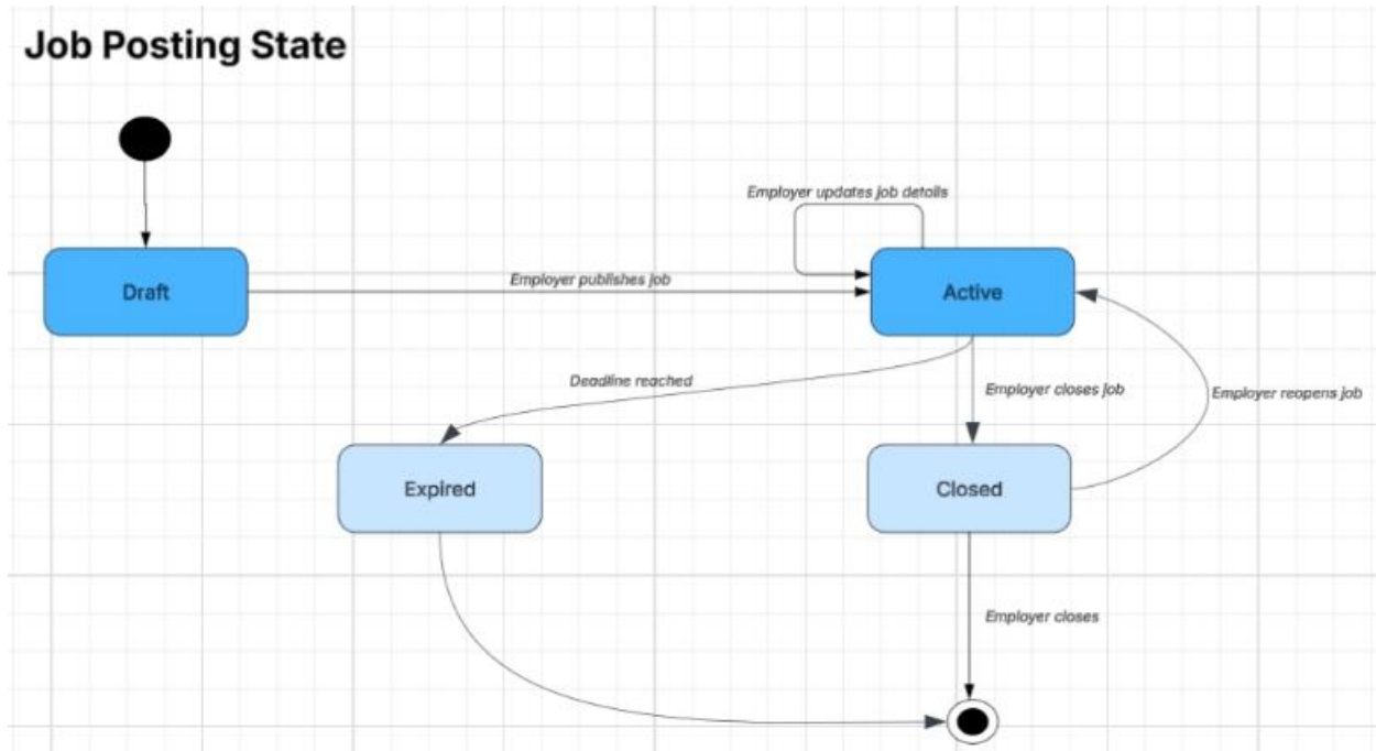
Figure 10: Job Posting State Diagram
