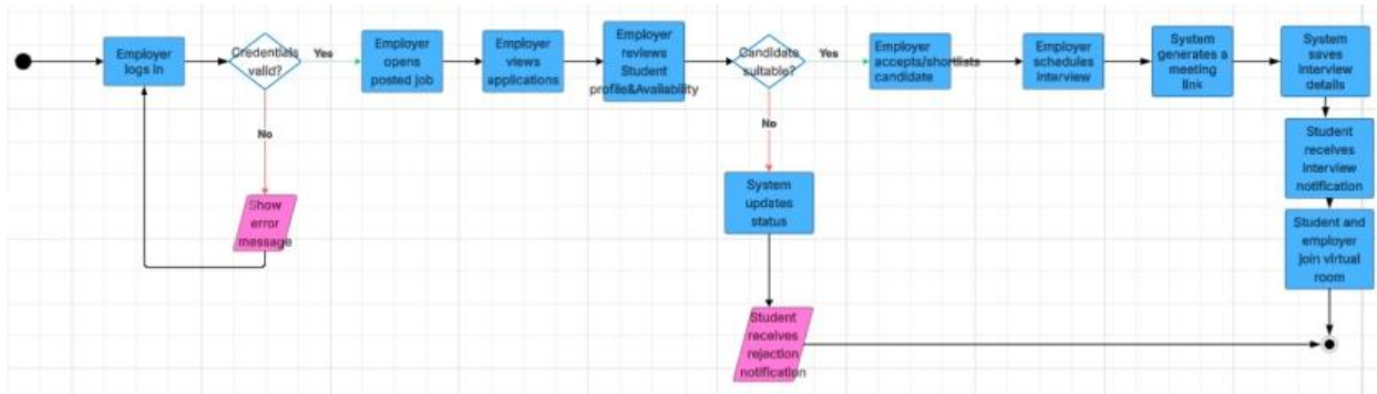
Figure 7: Activity diagram (Employers)
