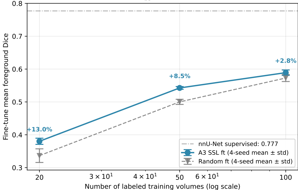
End-to-end fine-tune ( \text{lr}_{bb}=1\text{e-}4 ): A3 SSL vs Random init
