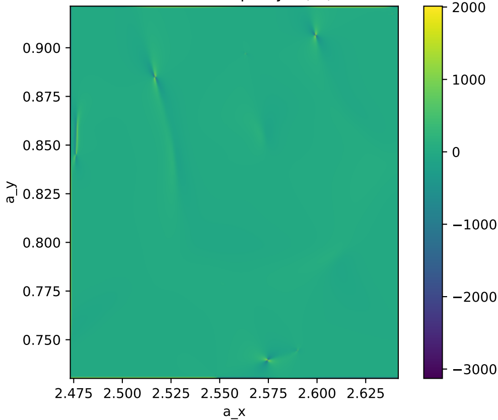
Handedness proxy \omega(t_0)
