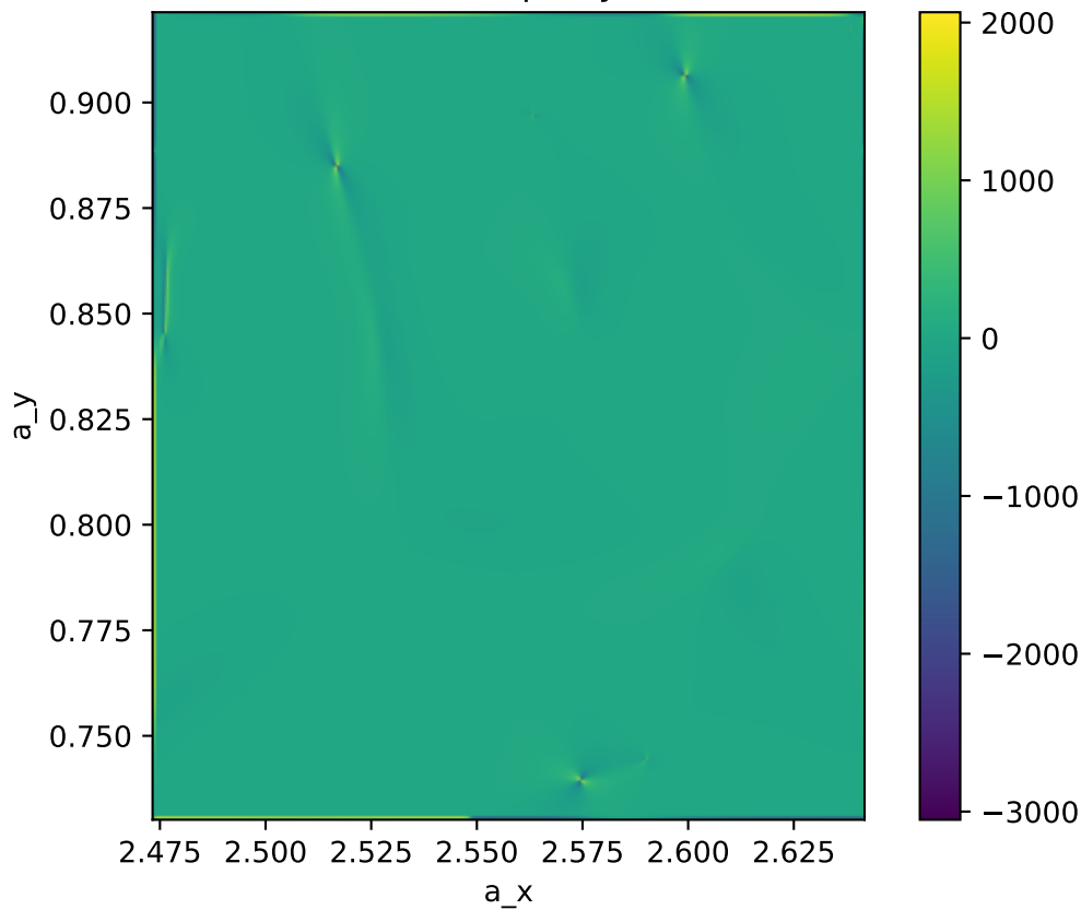
Handedness proxy \omega(t1)
