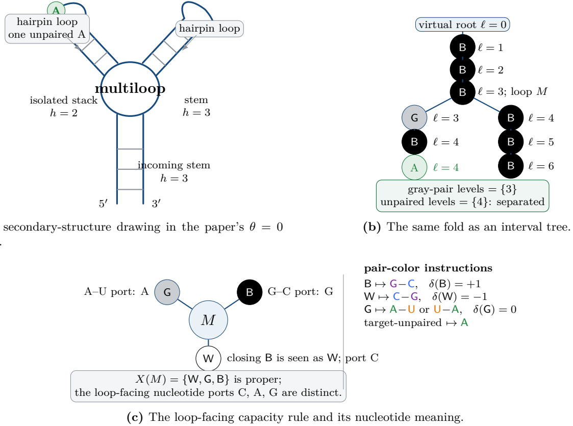
Figure 1: One RNA target in biological and mathematical representations. (a) The backbone drawing shows stems, hairpins, a multiloop, and an unpaired nucleotide. (b) Every target base pair becomes one colored tree node, every unpaired nucleotide becomes one leaf, and levels are root-path sums. (c) At the multiloop, the incoming black closing pair contributes its inverse white incidence. All pair markers carry explicit B, W, or G labels, so the figure does not rely on hue.
