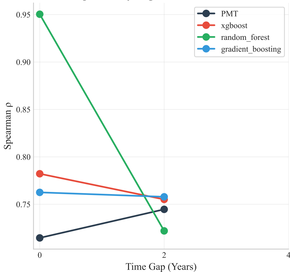
Spearman \rho Degradation Over Time
