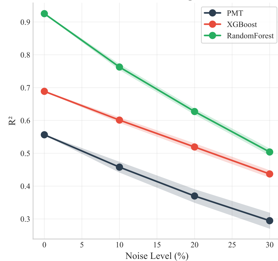
Robustness to Missing Noise
