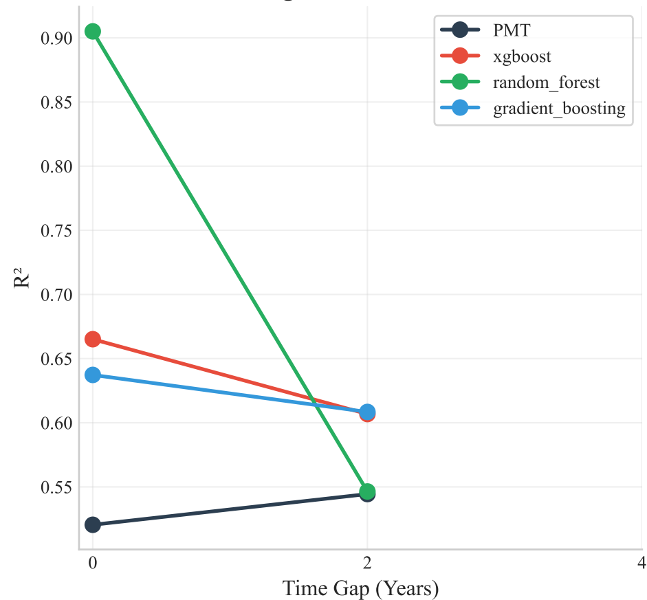
R 2 Degradation Over Time
