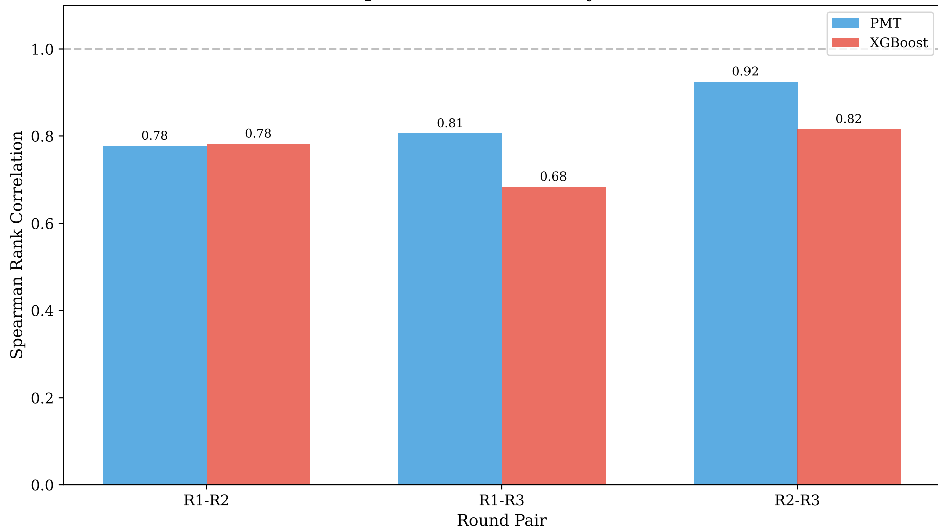
Feature Importance Rank Stability Across Rounds
