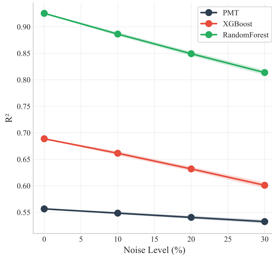
Robustness to Gaussian Noise
