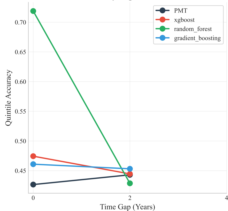
Quintile Accuracy Degradation Over Time
