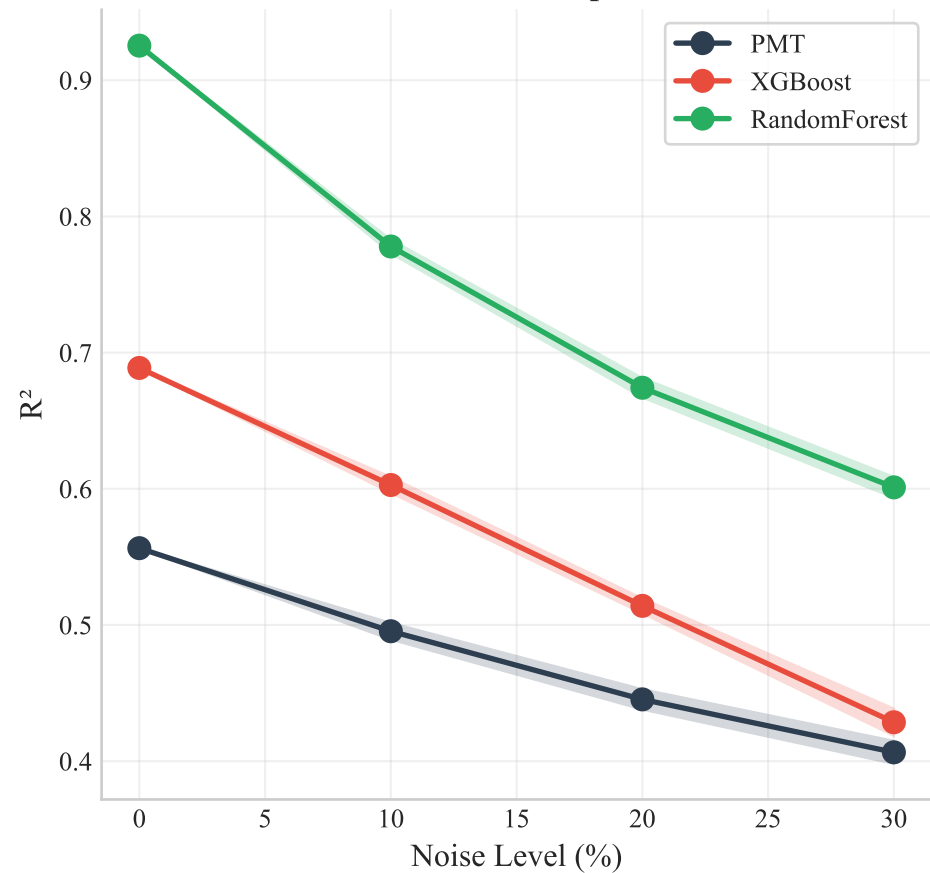
Robustness to Flip Noise
