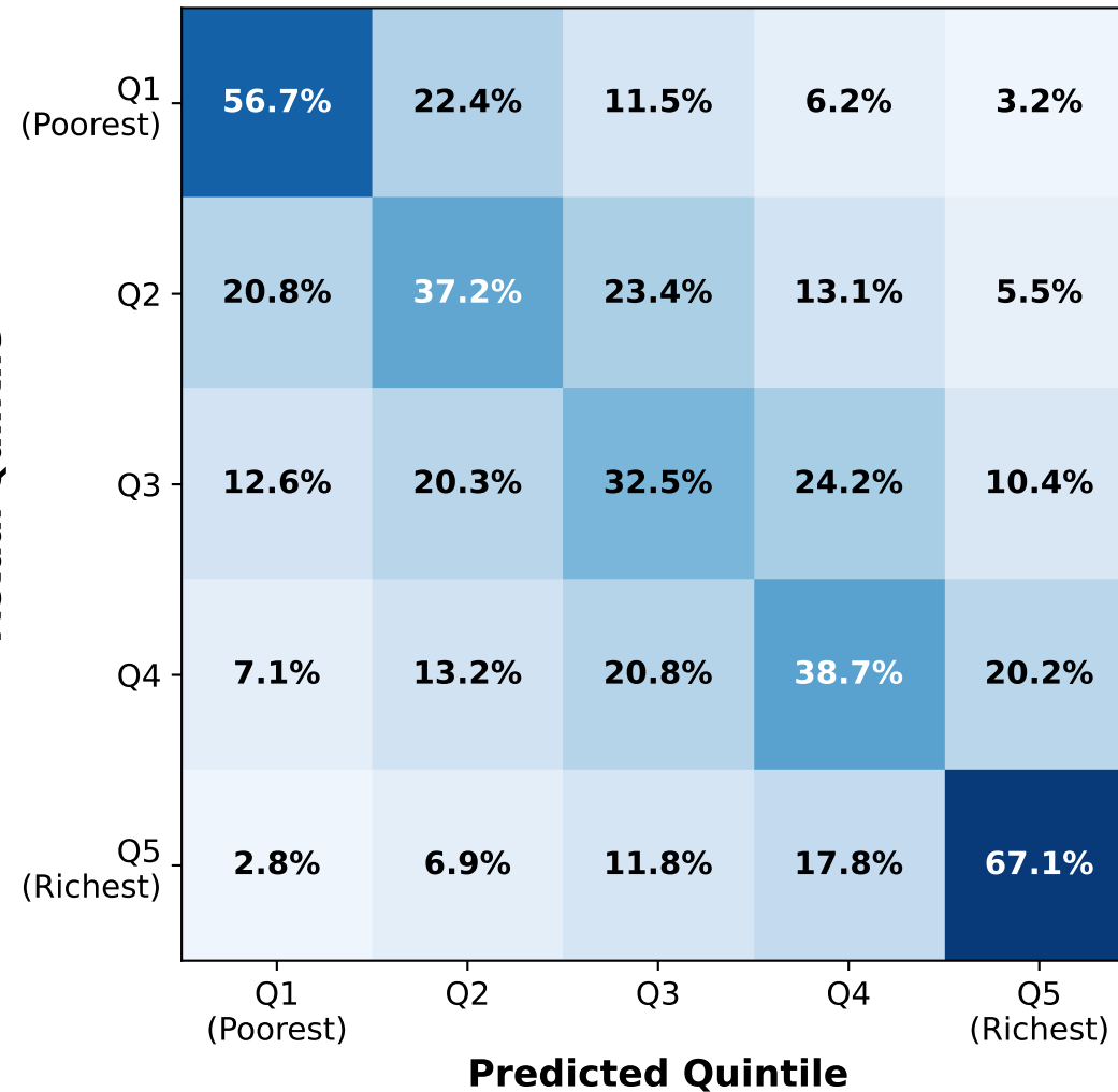
XGBoost (Machine Learning)
