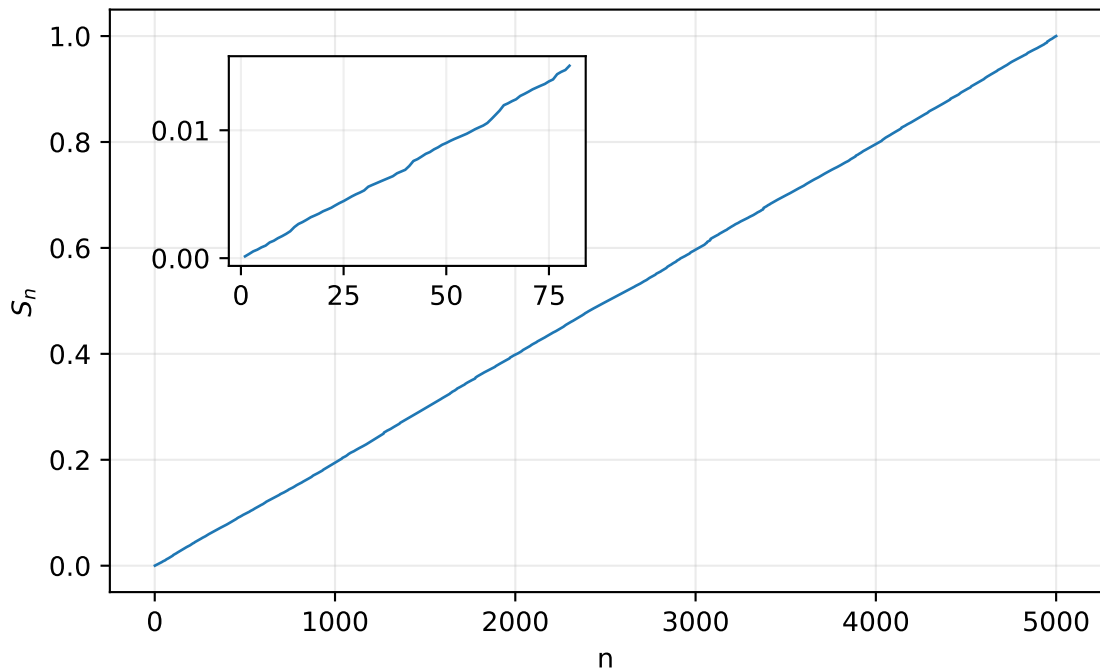
Pareto \mu = 3.0 , N=5000
