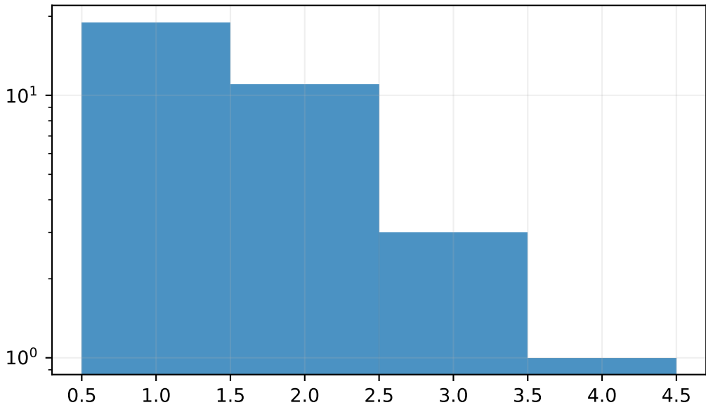
Recession durations
