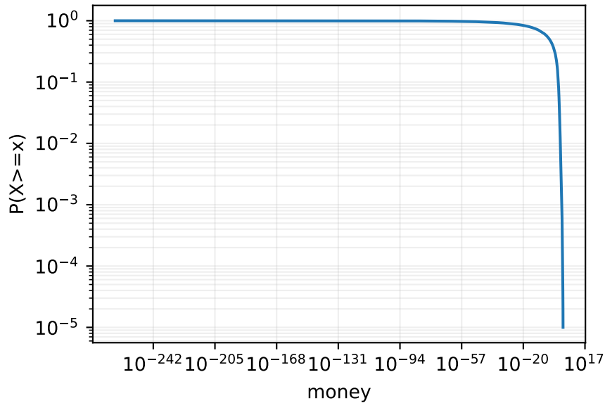
Wealth ccdf
