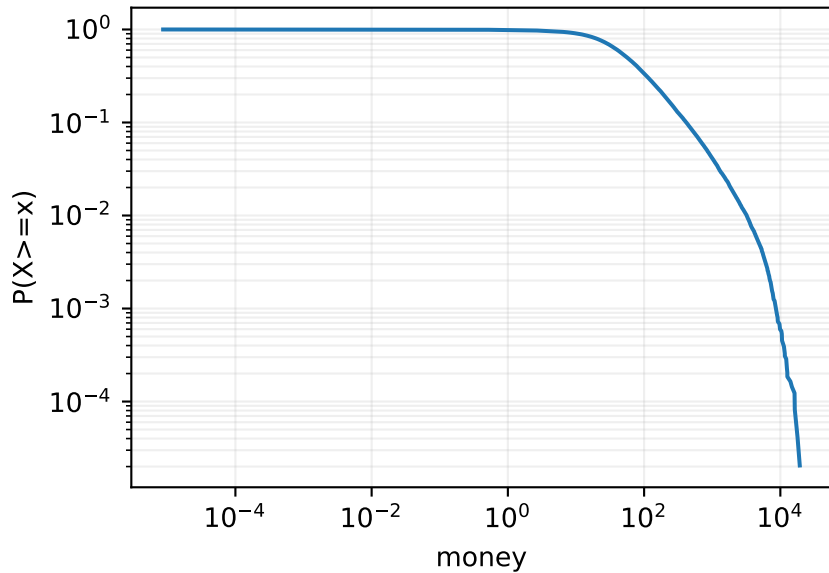
Income ccdf
