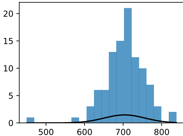
workers \mu=703.6 , sd=53.1
