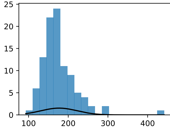
unemployed \mu=176.9 , sd=45.8
