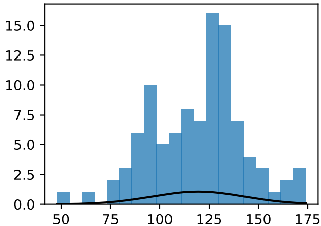
capitalists \mu=119.5 , sd=23.6
