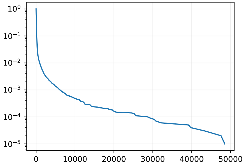
Money ccdf semi-log
