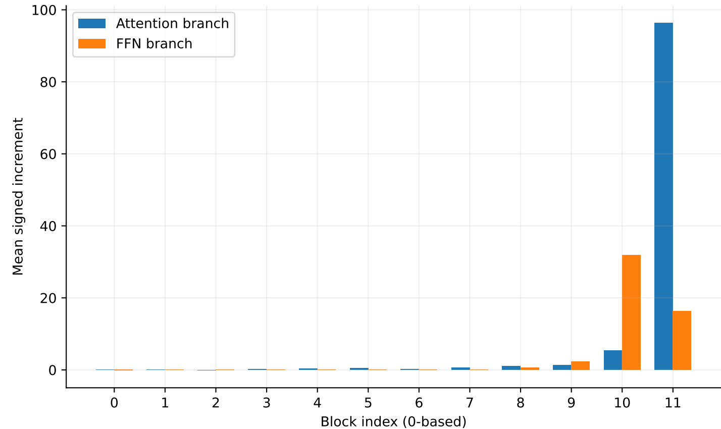
GPT-2 FP16: feature 496 mean additions
