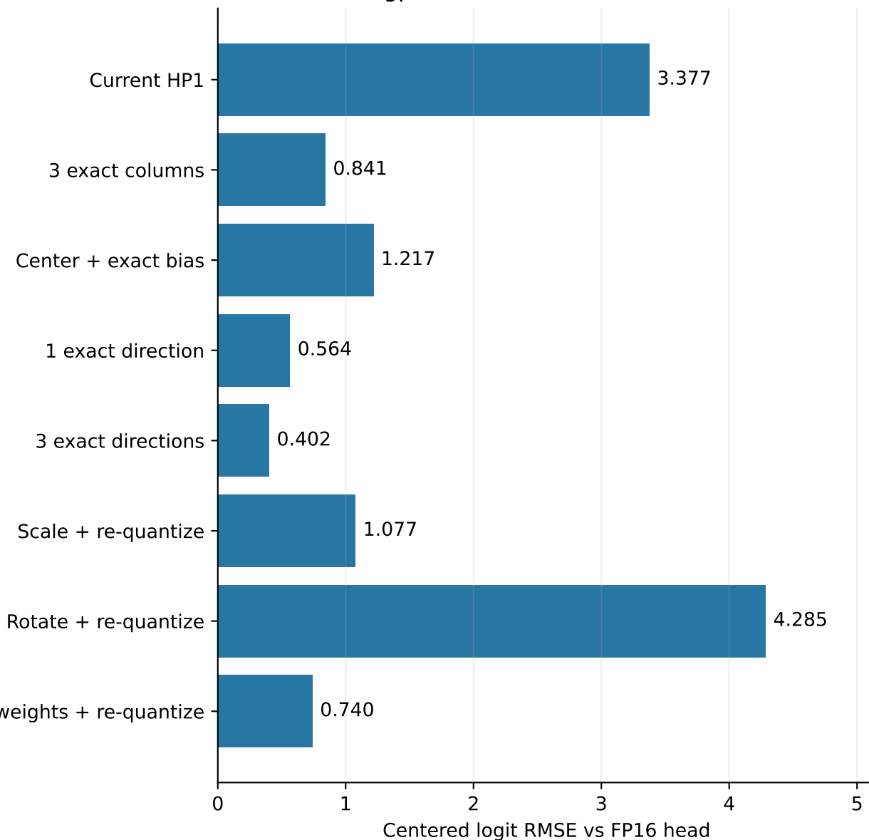
gpt2: current HP1 INT4 head
