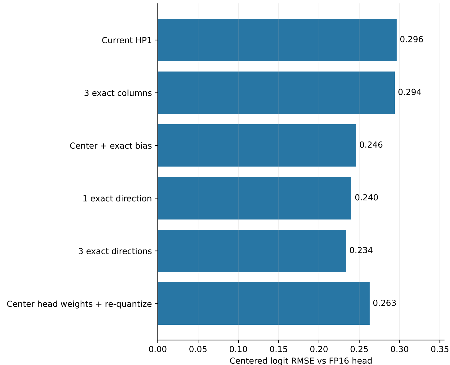
llama: current HP1 INT4 head
