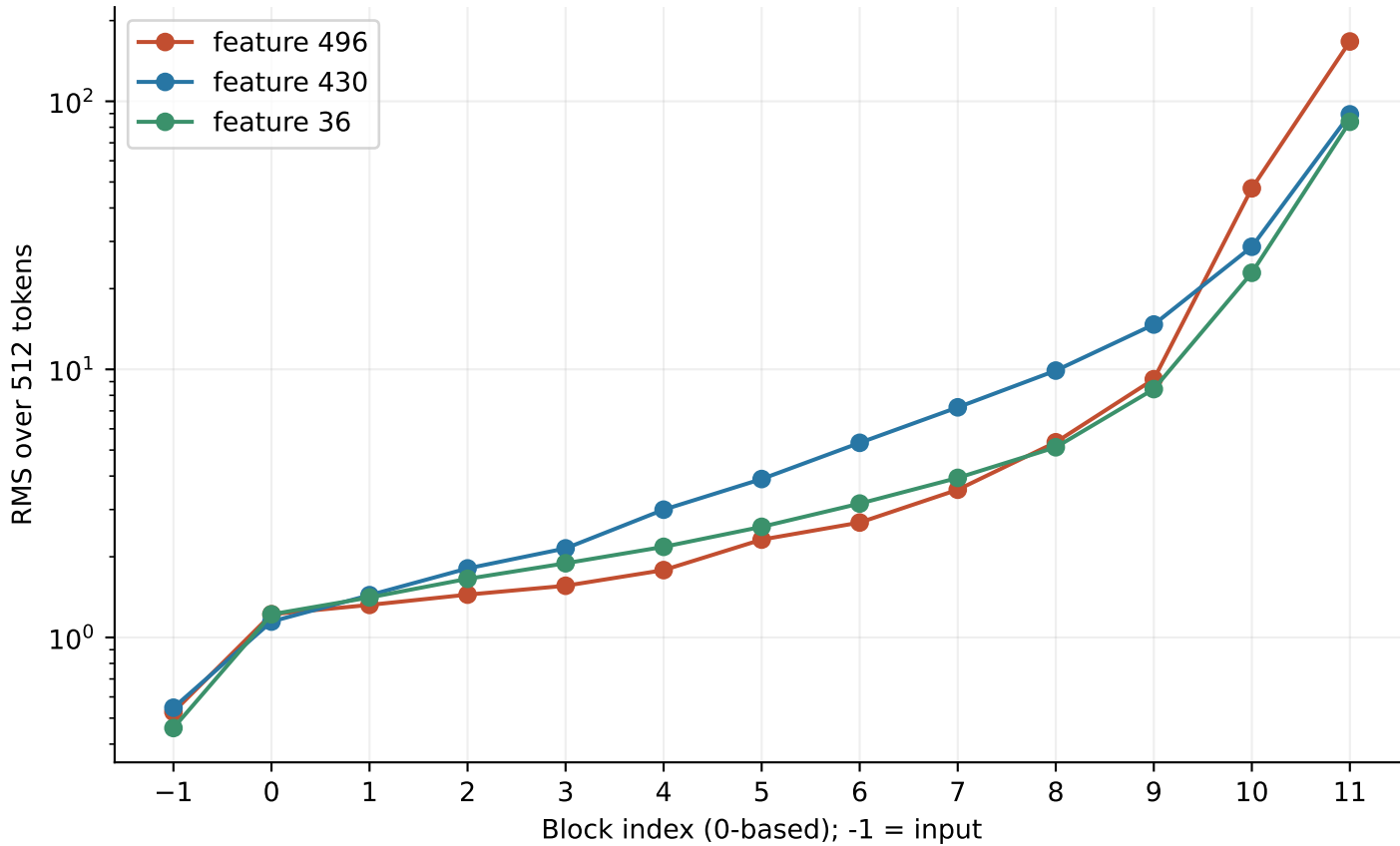
Final normalization: same 512-token traces
