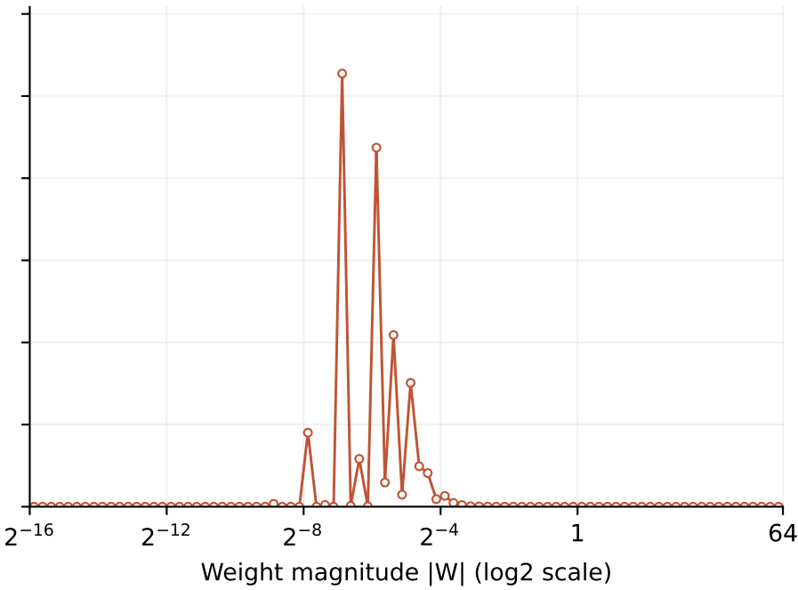
INT4 (Q4_HP1)
