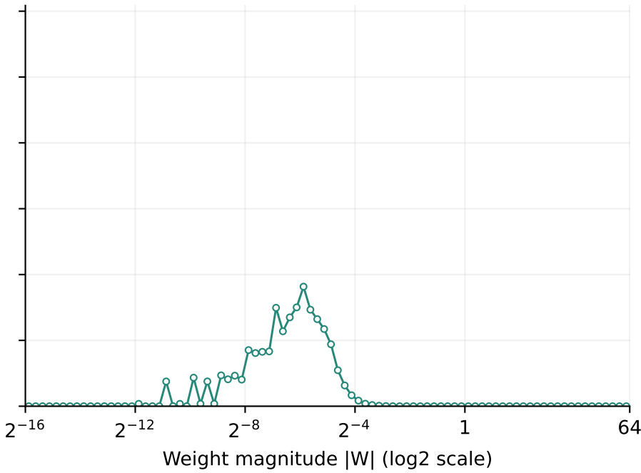
INT8 (Q8_HP1)
