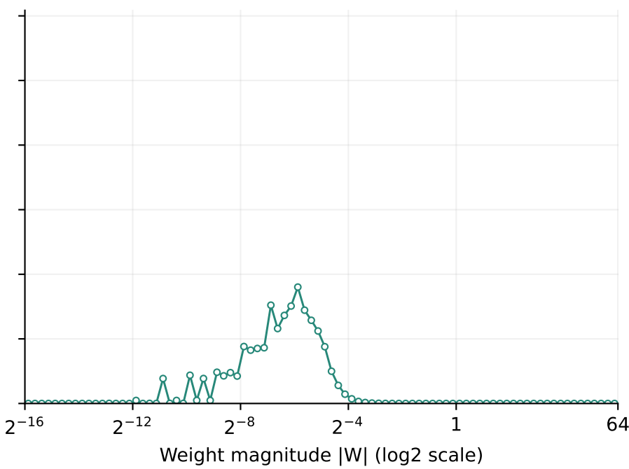
INT8 (Q8_HP1)
