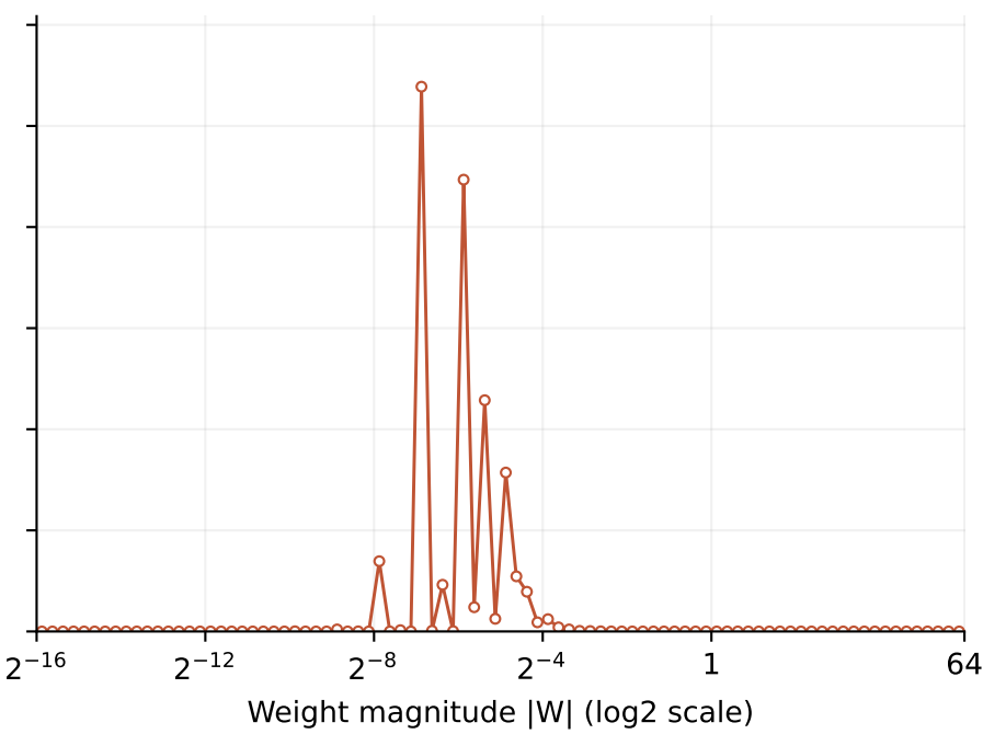
INT4 (Q4_HP1)
