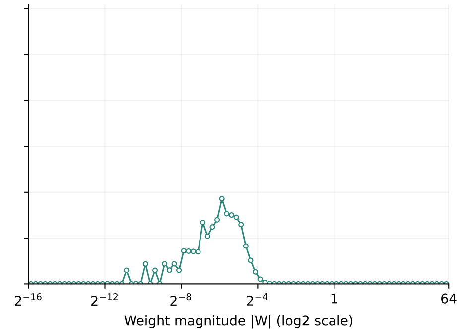
INT8 (Q8_HP1)
