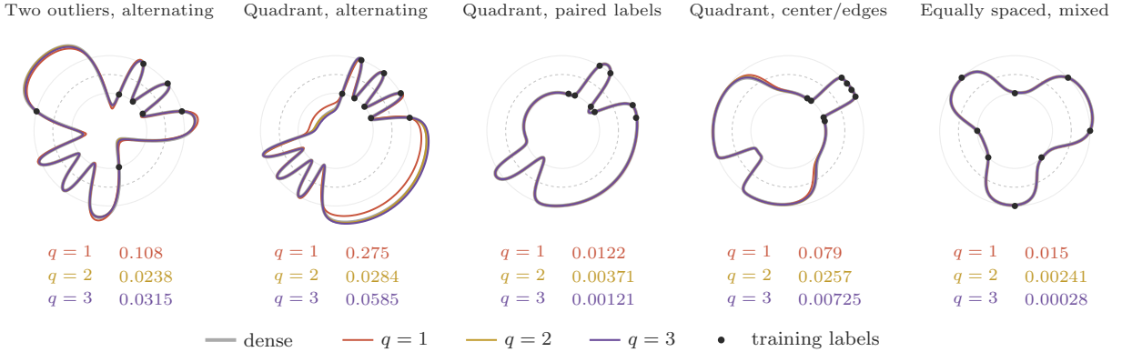
Figure 2: Fitted functions on unseen inputs. Existing five-task comparison: three hidden tanh layers, width 4096, and Legendre orders q = 1, 2, 3 , at each model’s own training-MSE 10^{-3} endpoint, not a shared time. Grey curves are dense predictions, coloured curves are memory predictions, and black points are labels. Printed discrepancies are RMS differences on 8192 circle queries, not uniform errors or risk against unseen labels. Fixed initialized matrices remain additional to Legendre’s moving state.
