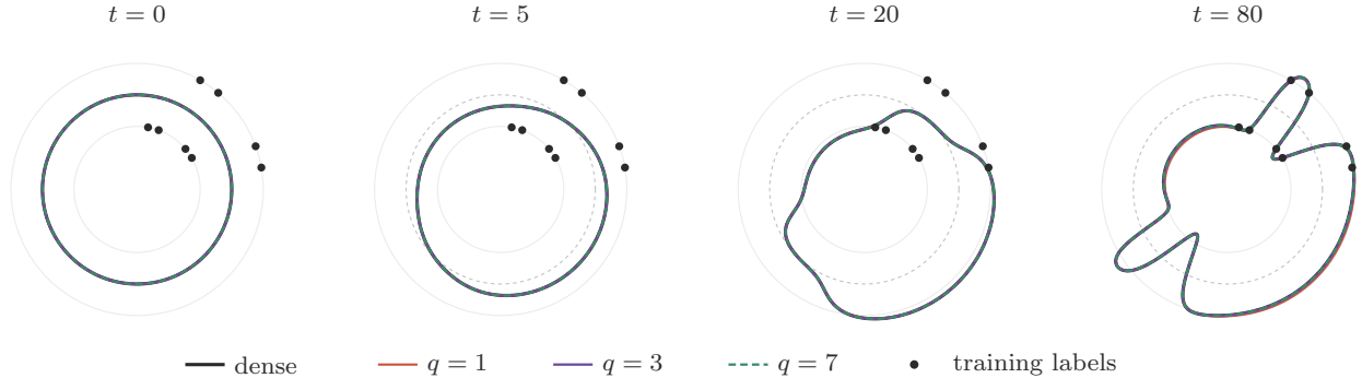
Figure 1: A trajectory, not only an endpoint. Existing paired-label circle experiment: two hidden tanh layers, width 2048, and Legendre orders q = 1, 3, 7 . Predictions are saved at the same physical times t = 0, 5, 20, 80 . Radius is 3 + f(\theta) , the dashed ring marks zero, and black points are training labels. The source replay records 39 common times and uses float64 adaptive Heun integration at two tolerances. These are discrete observations, not a certificate between the saved times.
