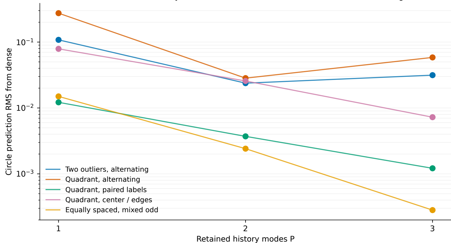
Three hidden tanh layers, width 4096 · each model at its own loss crossing
