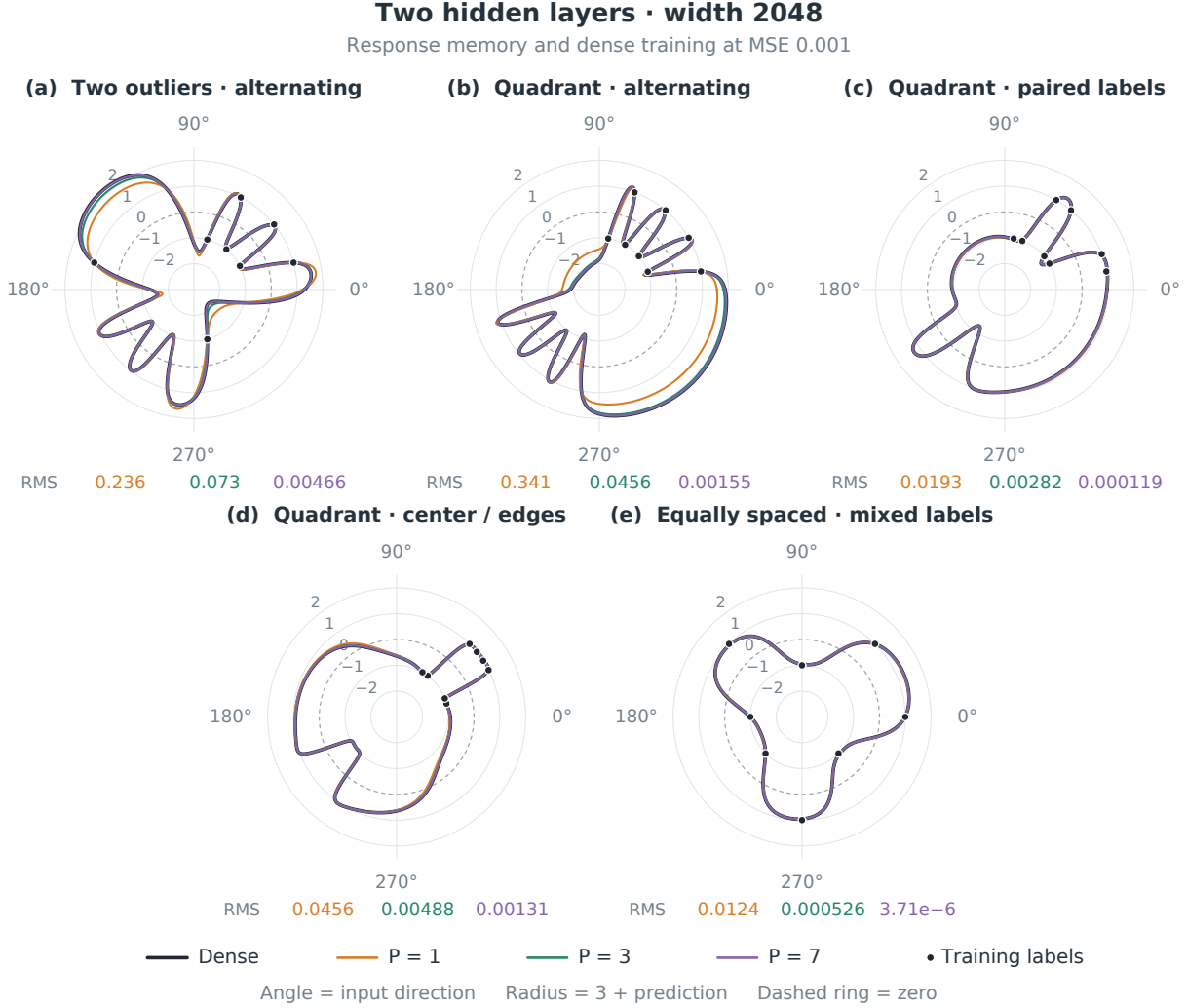
Figure 2: Fitted circle predictions for two hidden tanh layers, width 2048, and response-memory orders P = 1, 3, 7 , using the dense references in Table 2. Models are evaluated at their individual training-MSE 10^{-3} endpoints. Angle is input direction and radius is 3 + f(\theta) ; signed radial ticks, the dashed zero-output ring, black training labels, and dense-versus-memory RMS values follow Figure 1. RMS is measured on 8192 uniform circle points.
