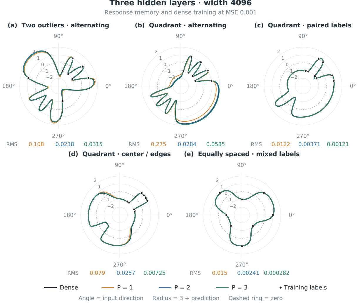
Figure 1: Fitted circle predictions for three hidden tanh layers, width 4096, and response-memory orders P = 1, 2, 3 , at each model’s training-MSE 10^{-3} endpoint. Angle represents input direction; radius is 3 + f(\theta) , with radial ticks labelled by f(\theta) and a dashed zero-output ring. Black curves show dense training, coloured curves show response memory, and black dots show training labels. Coloured numbers give RMS prediction differences from dense on 8192 uniform circle points, in legend order.
