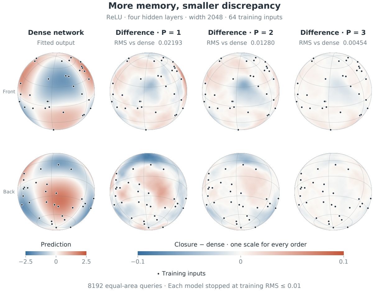
Figure 5: Saved fitted functions on the unit sphere for the target \sqrt{105} x_1 x_2 x_3 , with four hidden ReLU layers of width 2048 and 64 training inputs. The first column shows the dense output; the remaining columns show signed closure-minus-dense differences for P = 1, 2, 3 . Rows show complementary hemispheres, and black dots mark training inputs. Output colors use [-2.5, 2.5] ; every error panel uses [-0.1, 0.1] . Surface colors interpolate saved queries on a triangular mesh; RMS values use the original 8192 equal-area query values before interpolation. Models are compared at their individual training-RMS \leq 0.01 endpoints, using one network seed and float32 Euler steps of 1/128 . The order trend is specific to this one-seed comparison. These are fitted-function discrepancies, without a common-time trajectory comparison or a continuous-gradient-flow refinement certificate.
