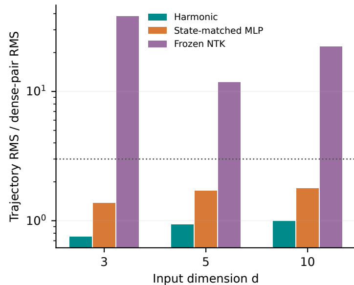
(a) Sphere checks, n = 2048
