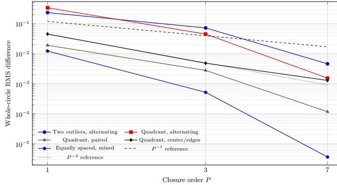
Figure 2: Whole-circle difference from dense training against order, two hidden tanh layers (left half of Table 1), with reference slopes. These are matched-loss discrepancies of fitted functions, not the same-time trajectory error bounded by Theorem 6.1.
