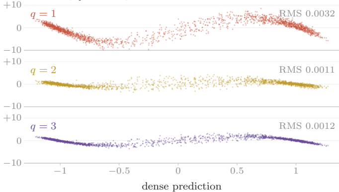
residual (f_q - f_{\text{dense}}) \times 10^3 , one shared scale
