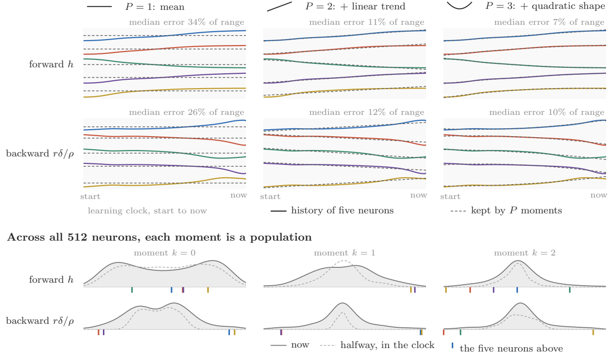
Figure 2: What Legendre moments retain of a history. A network with two hidden tanh layers of width 512 is trained by gradient descent on eight circle points, and the forward responses h and backward responses r\delta/\rho of one training input are recorded. Top: five neurons (one lane each) over the whole of training in the learning-speed clock, with their projections onto P = 1, 2, 3 Legendre modes (mean, linear trend, quadratic shape). These are projections fitted afterwards to the recorded dense histories, not trajectories of the closure. Above each panel, the median over all 512 neurons of the RMS projection error divided by the range of that neuron’s history. Bottom: across neurons each moment is a population; its distribution for the history up to the midpoint of the learning clock and for the whole history, with the five neurons above marked.
