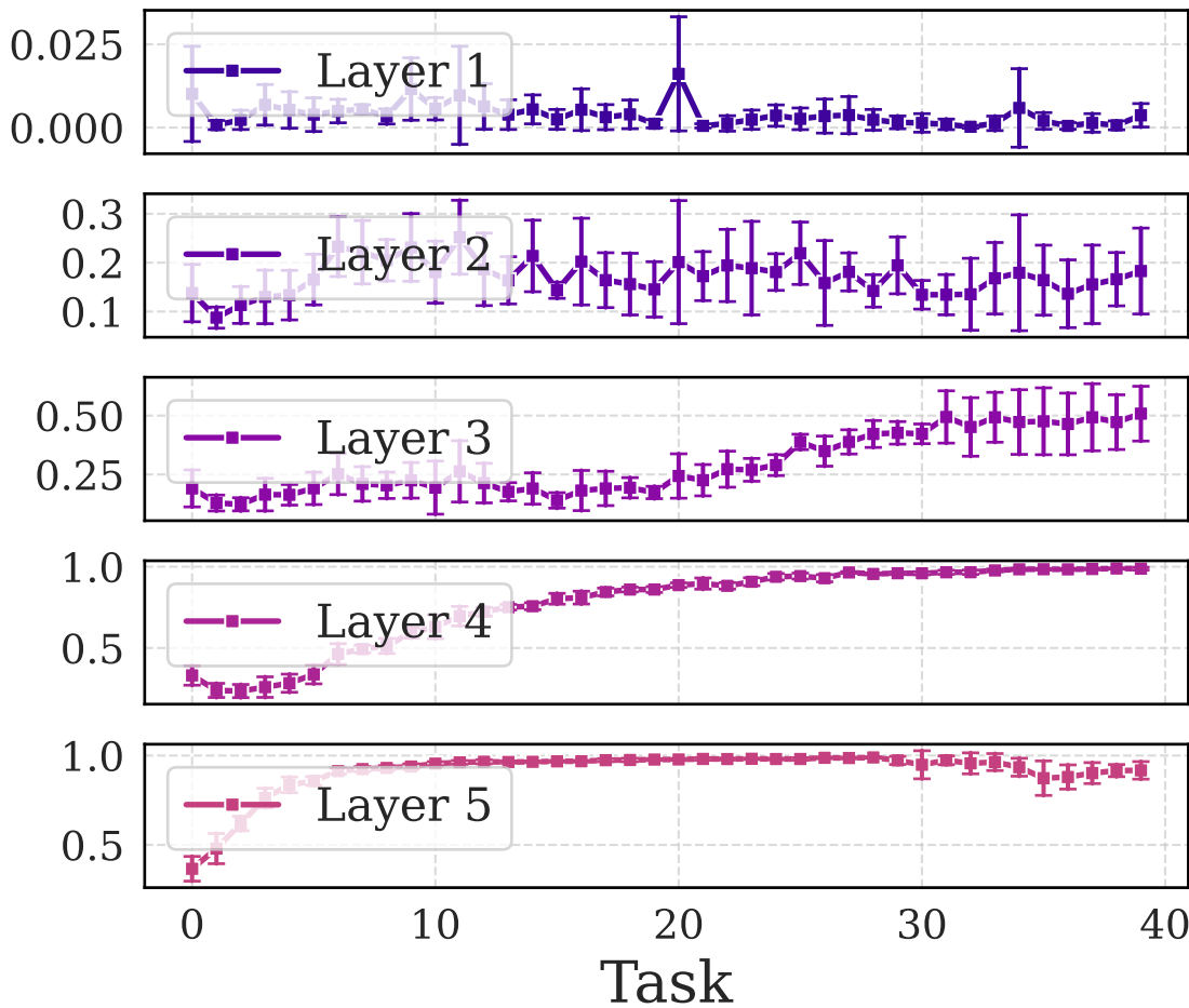
MLP Dead fraction
