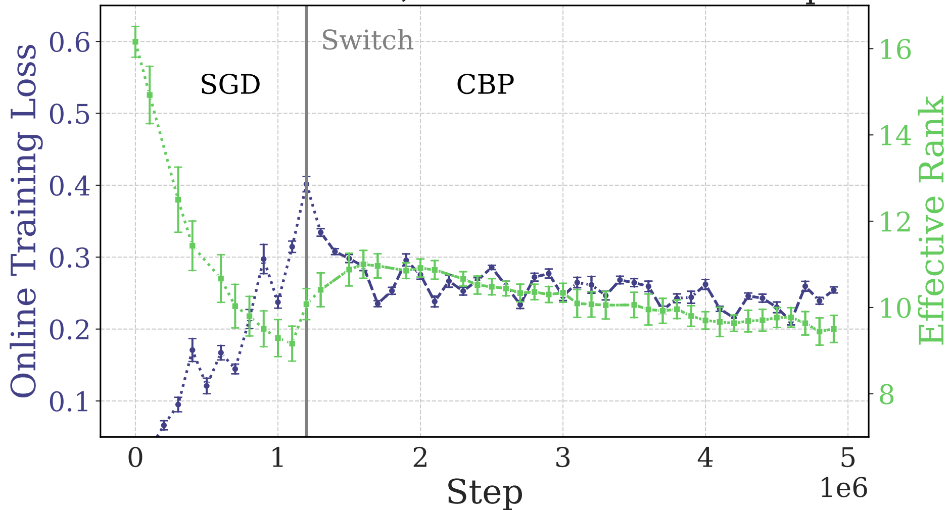
SGD first 25.0%, CBP second 75.0% steps
