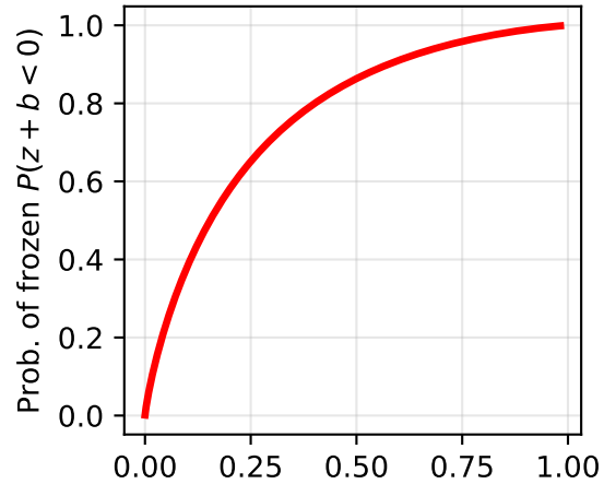
ReLU: varying bias
