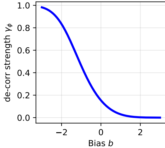
ReLU: Coefficient vs. Bias
