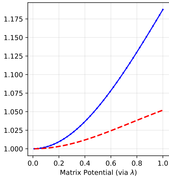
GELU Rank Gain
