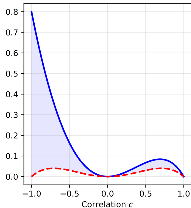
GELU Rank Gain
