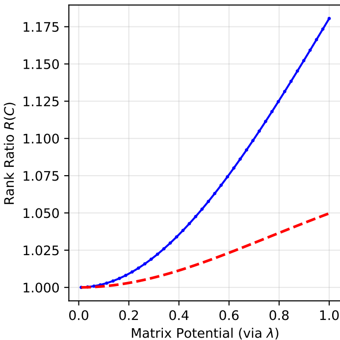
ReLU Rank Gain
