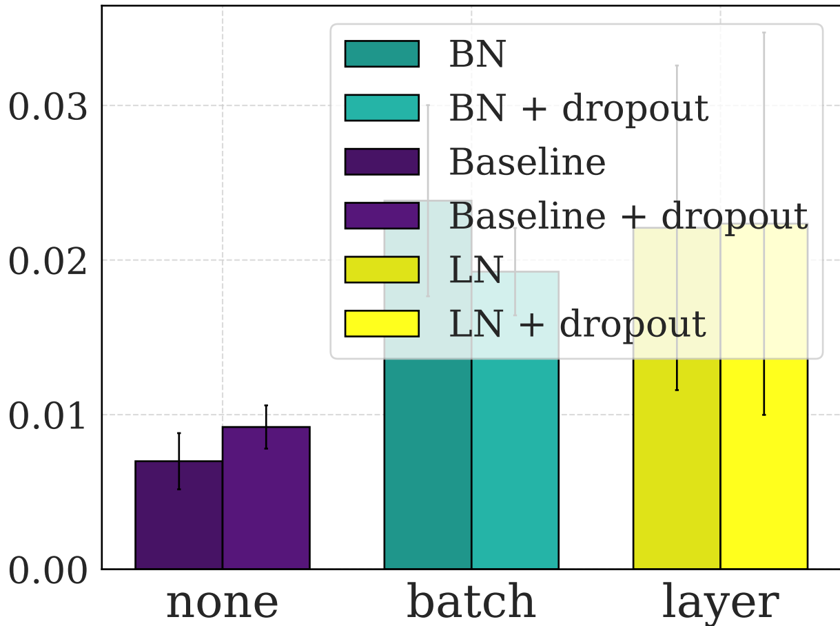
Duplicate Fraction
