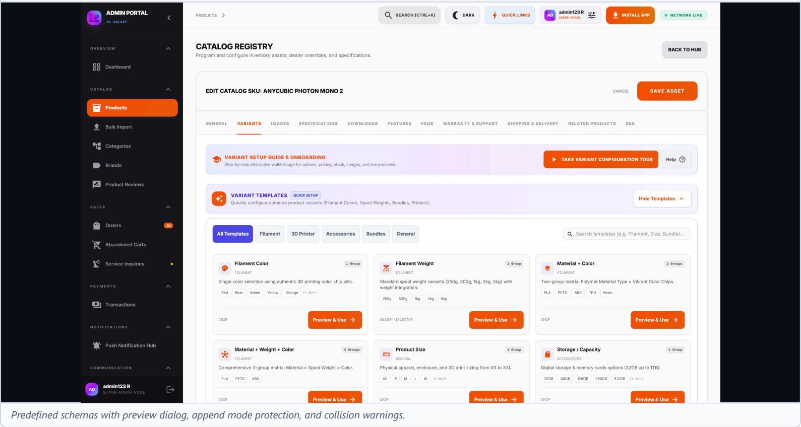
Figure 7.1 — Dynamic Variant Templates Library
