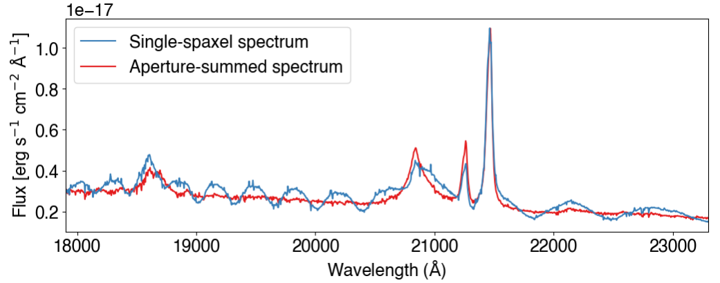
Figure 1: Illustration of the wiggles in the single-spaxel spectrum (blue), which is a manifestation of the resampling noise in the standard-pipeline-reduced datacube due to PSF undersampling. The orange spectrum shows the aperture-summed spectrum within a 4-spaxel radius. The illustrated data are of an active galactic nucleus (AGN) from Perna et al. (2023).
