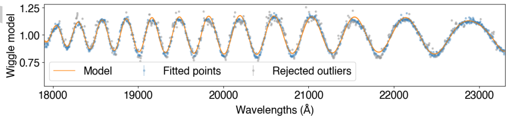
Figure 3: Illustration of the extracted and modeled wiggle signal. The illustrated data points represent D(\lambda)/M(\lambda) based on the best-fit M(\lambda) , and the orange line illustrates the best-fit wiggle model W(\lambda) . The grey points are rejected outliers using the false discovery rate method, and the blue points mark the wavelengths where the data were fit to the model.
