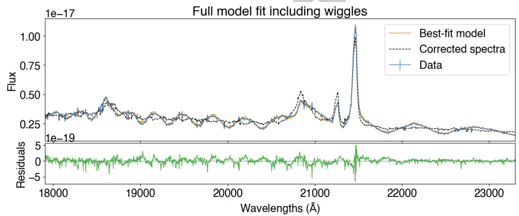
Figure 2: Modeling of the full spectrum (blue in the top panel) based on the template spectra and the wiggles impacting it. The illustrated spectrum is the same one from Figure 1. The best-fit model is shown in orange and the wiggle-corrected spectrum is shown in black. The bottom panel illustrates the residuals (green) between the original data and the best-fit model.
