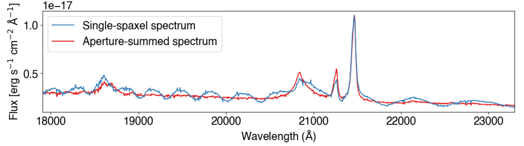
Figure 1: Illustration of the wiggles in the single-spaxel spectrum (blue), which is a manifestation of the resampling noise in the standard-pipeline-reduced datacube due to PSF undersampling. The red spectrum shows the aperture-summed spectrum within a 4-spaxel radius, normalized to match its maximum to that of the single-spaxel one. The illustrated data are of an active galactic nucleus (AGN) from Perna et al. (2023).
