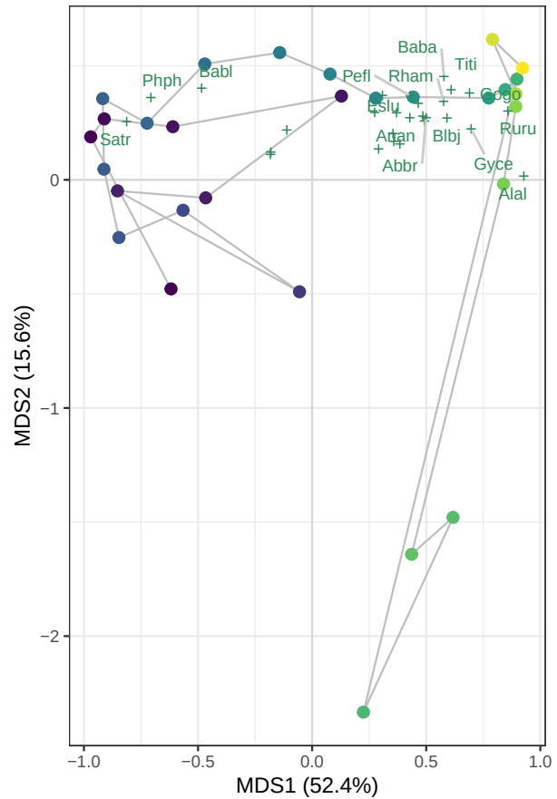
PCoA, Bray-Curtis
