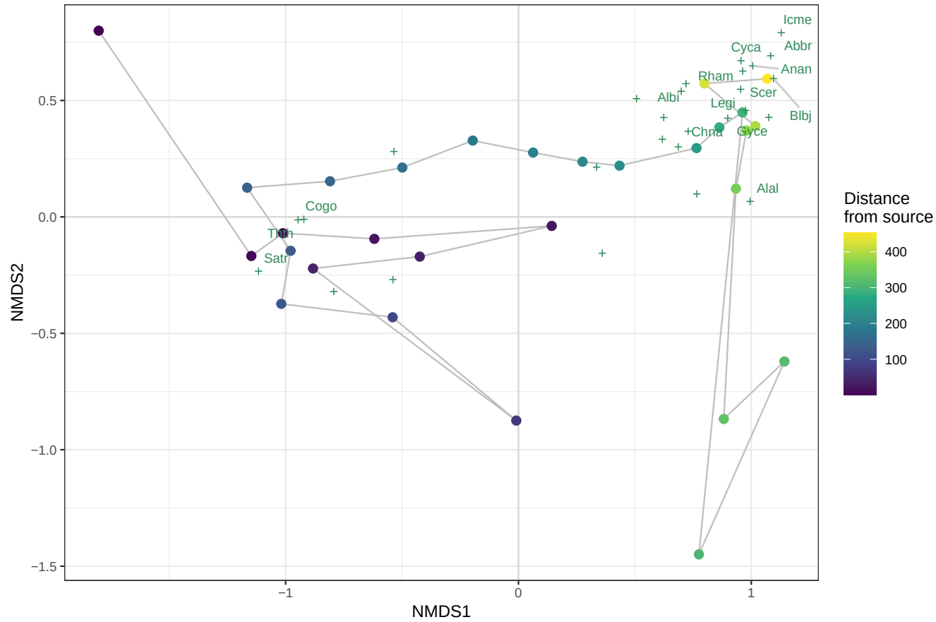
nMDS, stress = 0.075
