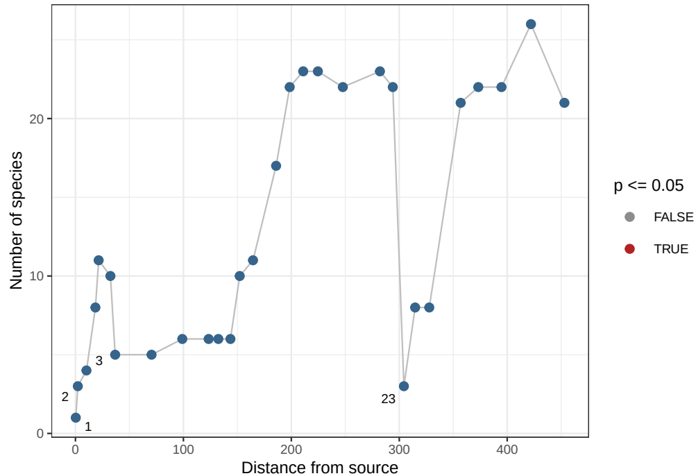
Species richness
