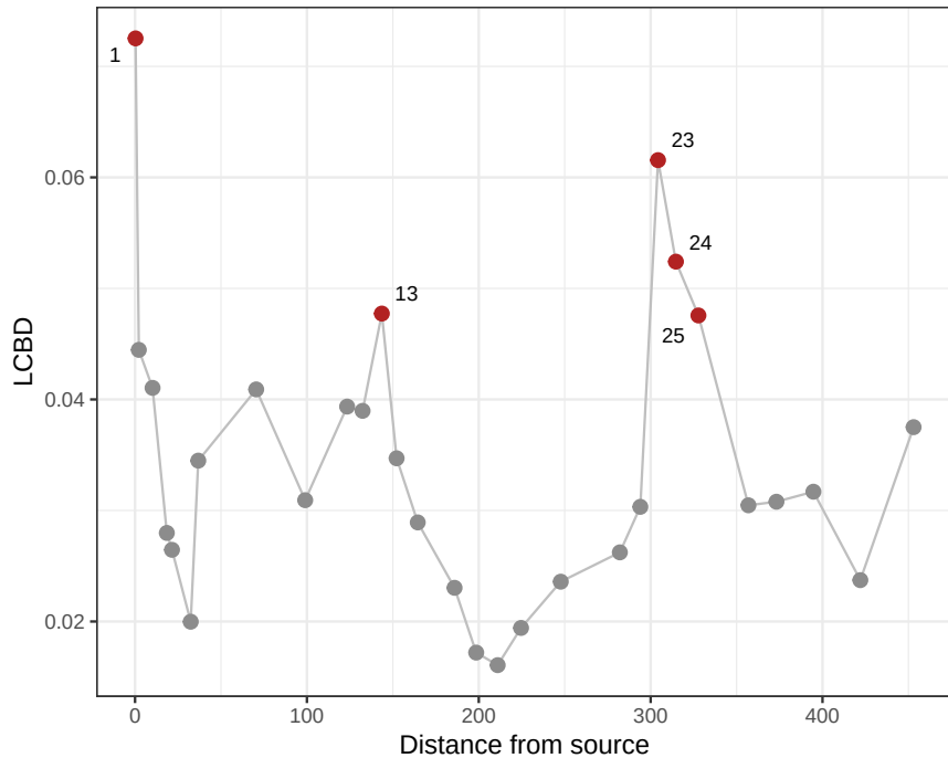
Local contribution to beta diversity
