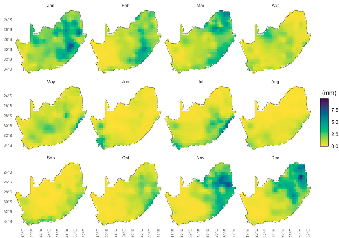
Figure 2: Figure 2. Mean monthly rainfall over South Africa for the year 2016.
