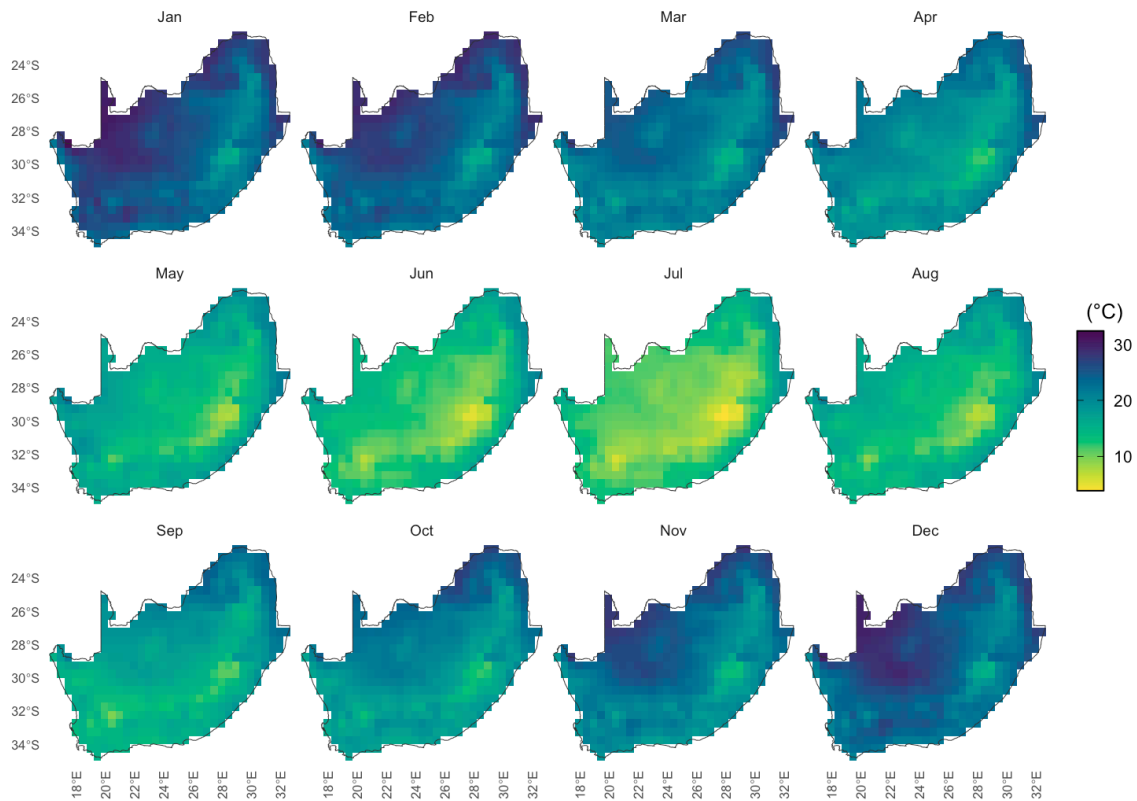
Figure 1: Figure 1. Mean monthly temperature over South Africa for the year 2016.
