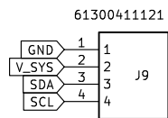
OLED SCREEN CONNECTOR
