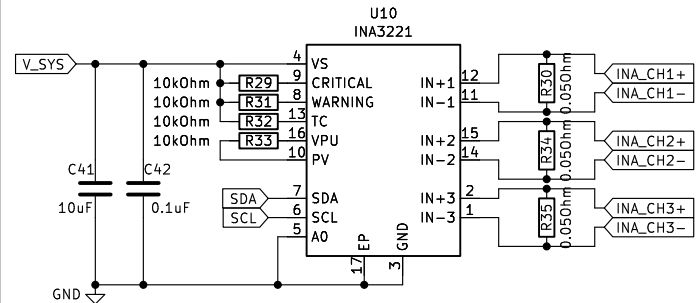
INA3221 CURRENT SENSOR
