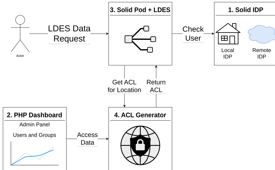
Figure 2: MuMo deployment overview with four components, an Identity Provider, a dashboard, a solid pod with the LDES publications, and an ACL file generator.
