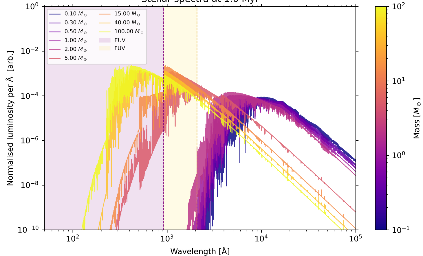
Stellar spectra at 1.0 Myr
