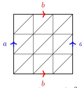
a triangulation of T^2
