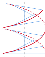
helicoid
