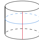
parabolic: K = 0
