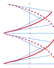
helicoid
