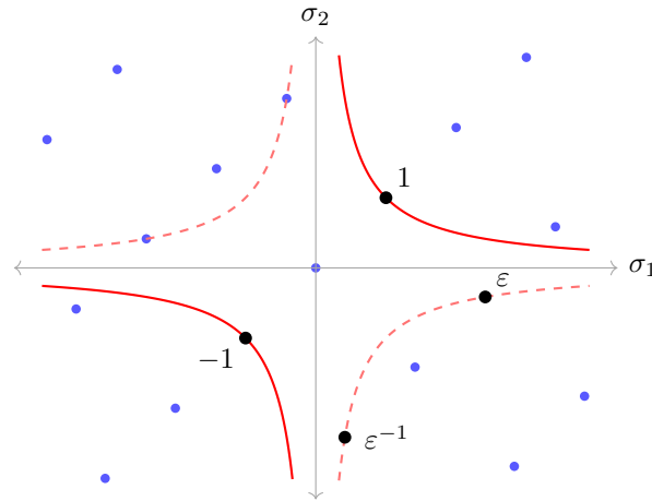
\sigma(\mathbb{Z}[\sqrt{2}]) and the hyperbolas y_1 y_2 = \pm 1
