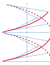
helicoid
