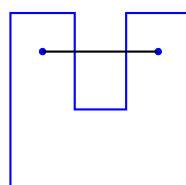
not convex
