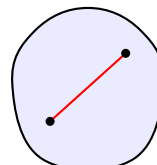
convex
