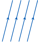
uniform flow
