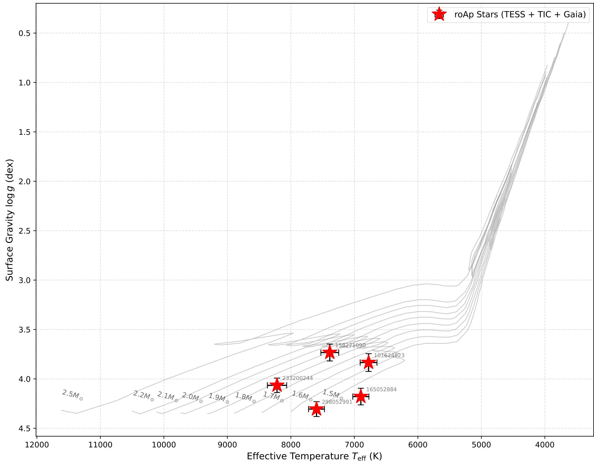
Hertzsprung-Russell Diagram: roAp Stars
