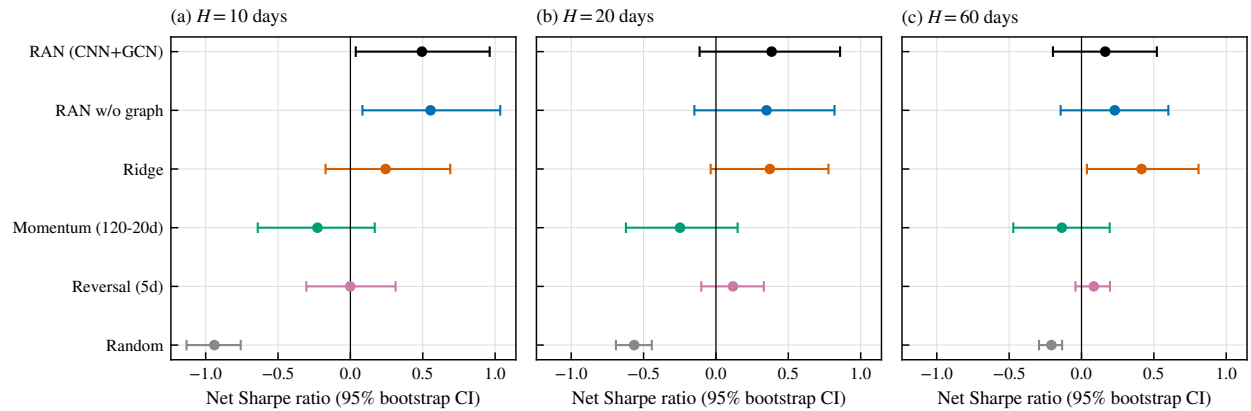
Figure 10: Sharpe-ratio comparison across S&P 500 models and horizons. The figure is descriptive and uses the saved development-stage outputs.
