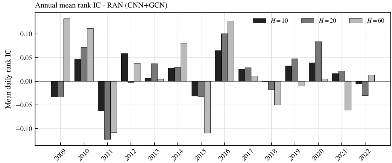
Figure 12: Annual rank IC for the S&P 500 RAN configurations. The figure is descriptive and uses the saved development-stage outputs.
