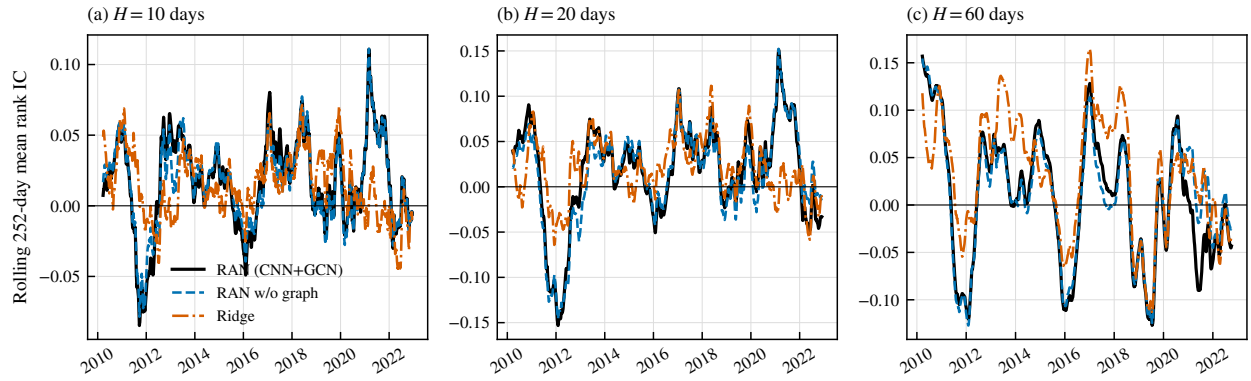
Figure 9: Rolling rank IC for the S&P 500 development experiment. The figure is descriptive and uses the saved development-stage outputs.
