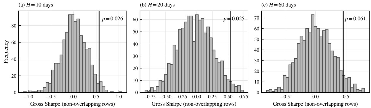
Figure 13: Permutation null distributions for the S&P 500 RAN results. The figure is descriptive and uses the saved development-stage outputs.
