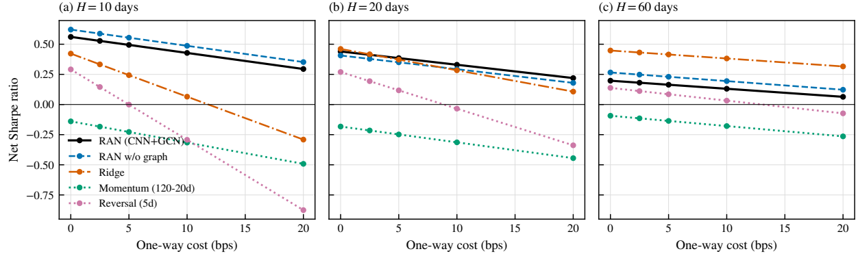
Figure 11: Transaction-cost sensitivity of net Sharpe on the S&P 500 universe. The figure is descriptive and uses the saved development-stage outputs.
