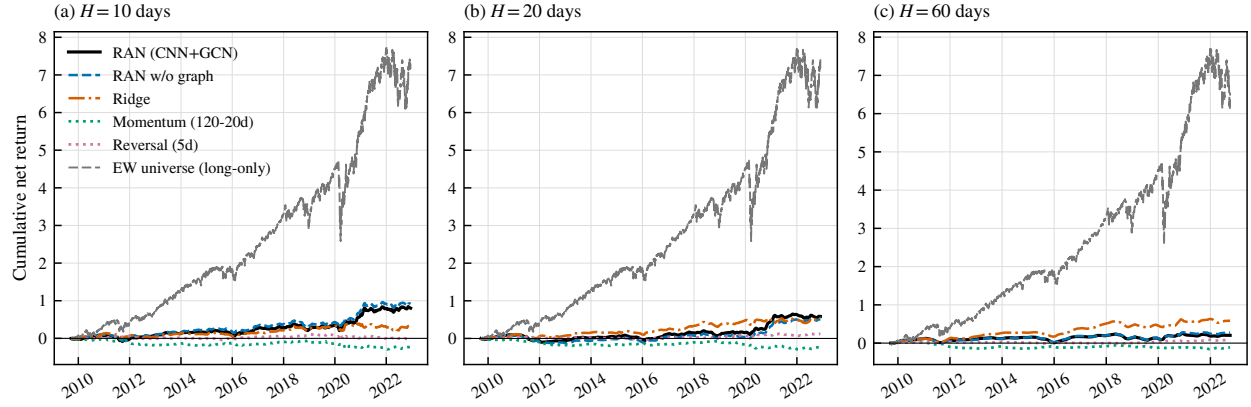
Figure 8: Cumulative net return for the S&P 500 development experiment. The figure is descriptive and uses the saved development-stage outputs.
