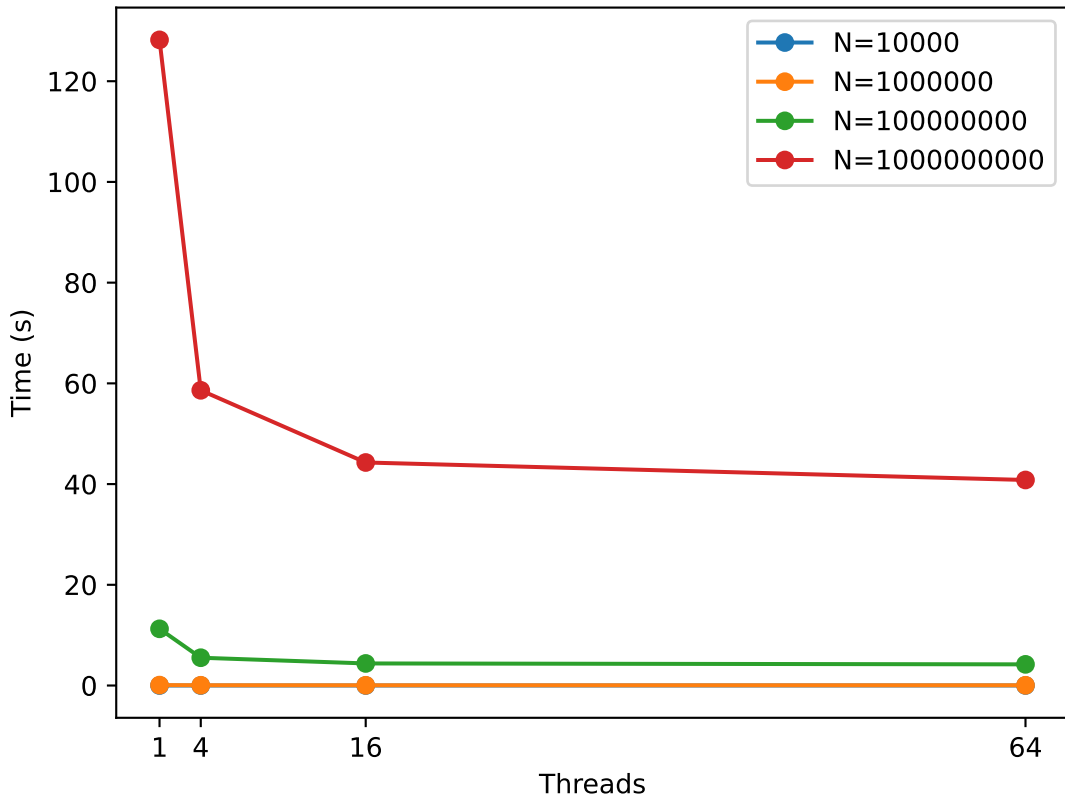
Merge Sort: Parallel Time vs Threads
