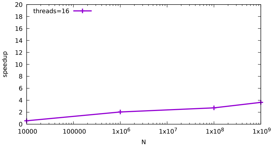
mergesort- 16 threads
