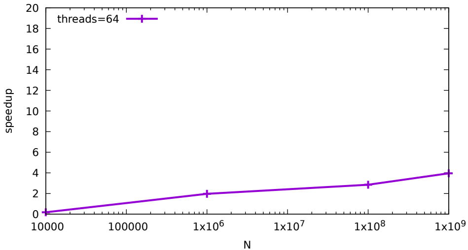
mergesort- 64 threads
