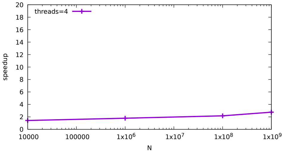
mergesort- 4 threads
