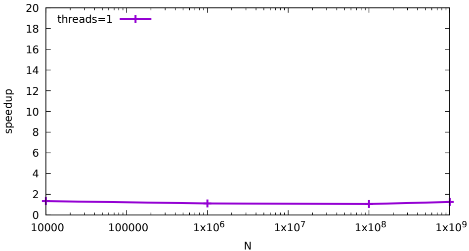
mergesort- 1 threads
