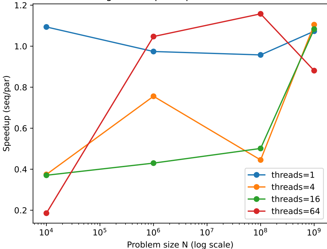
Merge Sort: Speedup vs Problem Size
