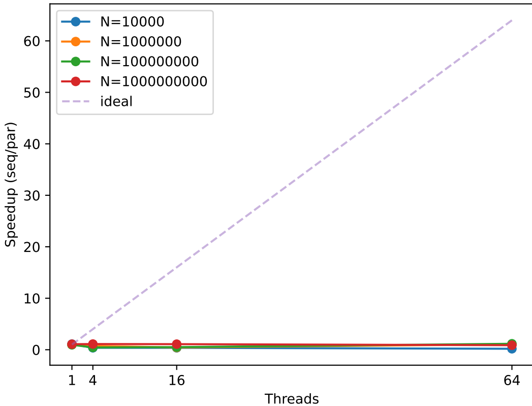
Merge Sort: Speedup vs Threads
