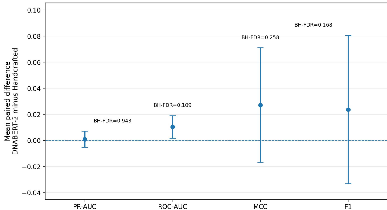
Paired Metric Differences Across Repeated Splits
